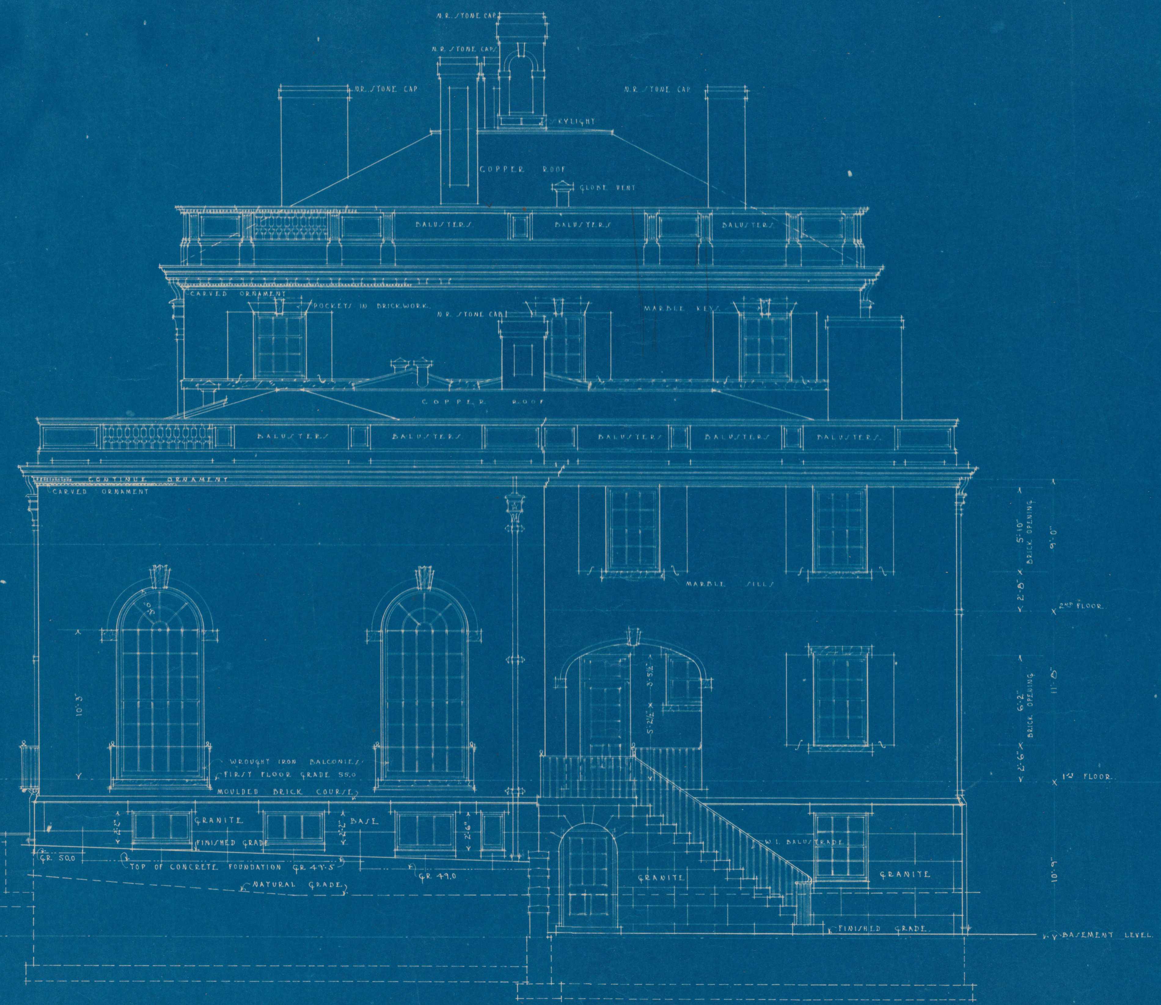
NORTH ELEVATION SCALE 1/4" = 1'-0"
