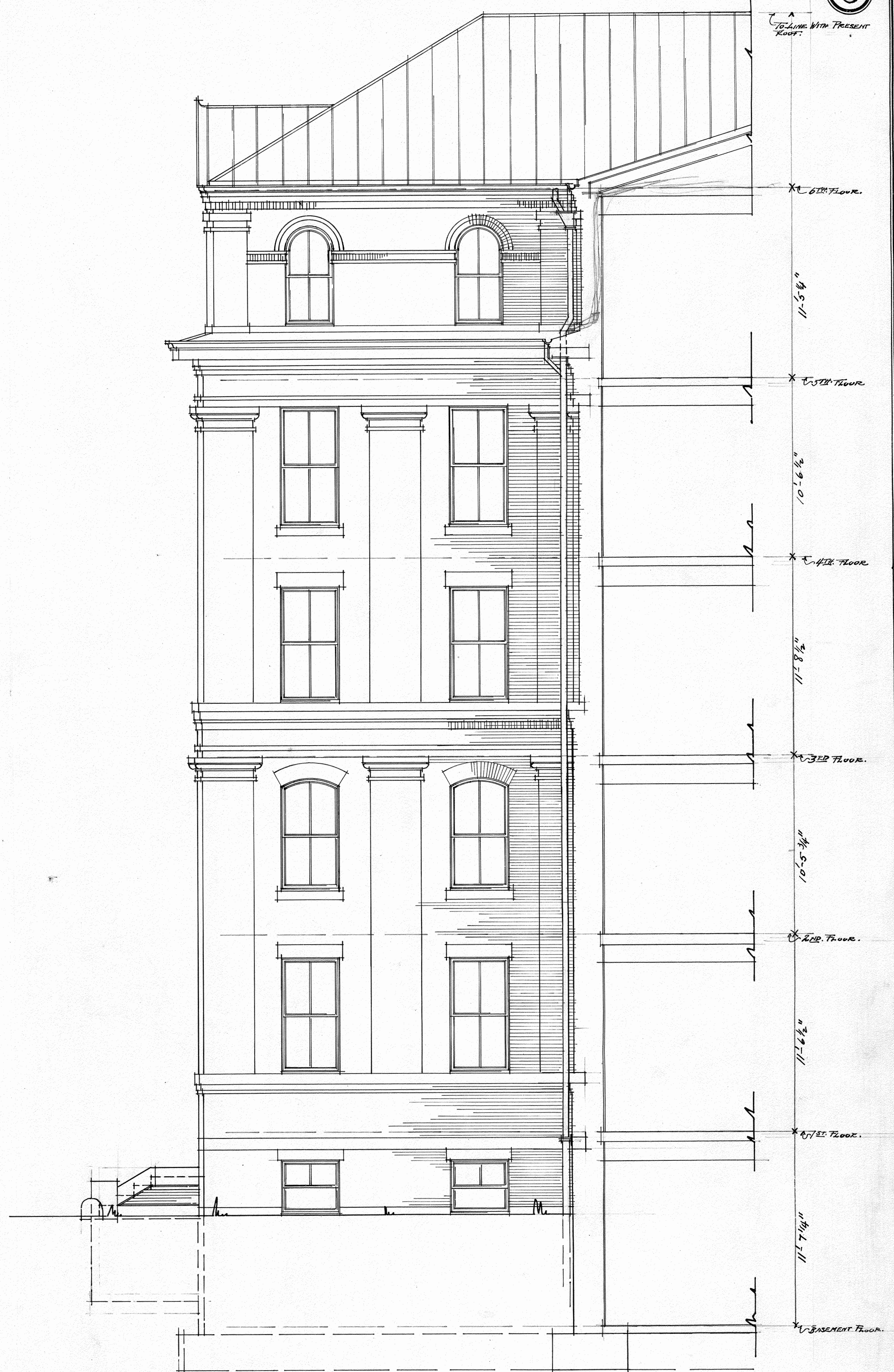
SIDE ELEVATION OF ENTRANCE BAY
