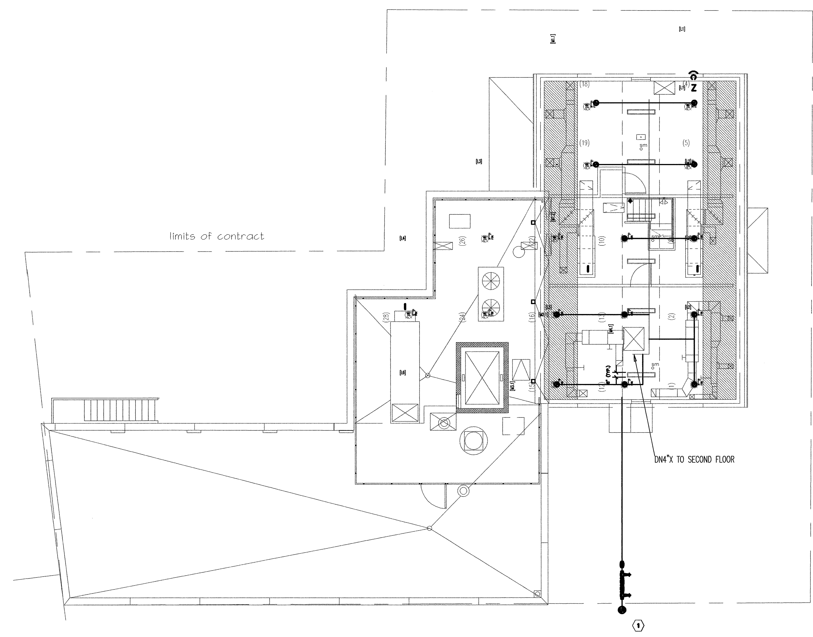
Attic Floor Sprinkler Plan
