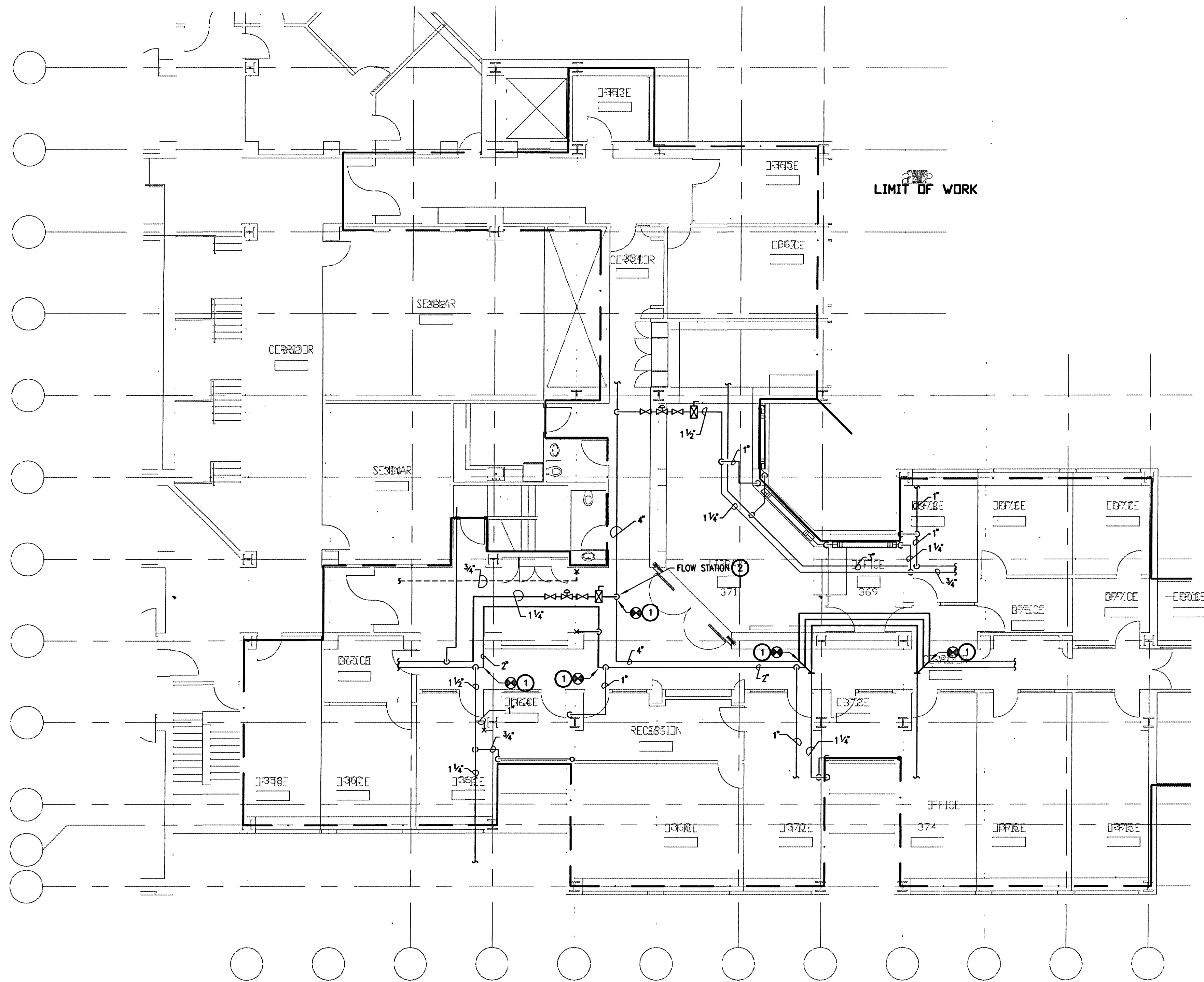
HVAC PIPING REVISIONS PART-PLAN SCALE: 1/8"=1'-0"
