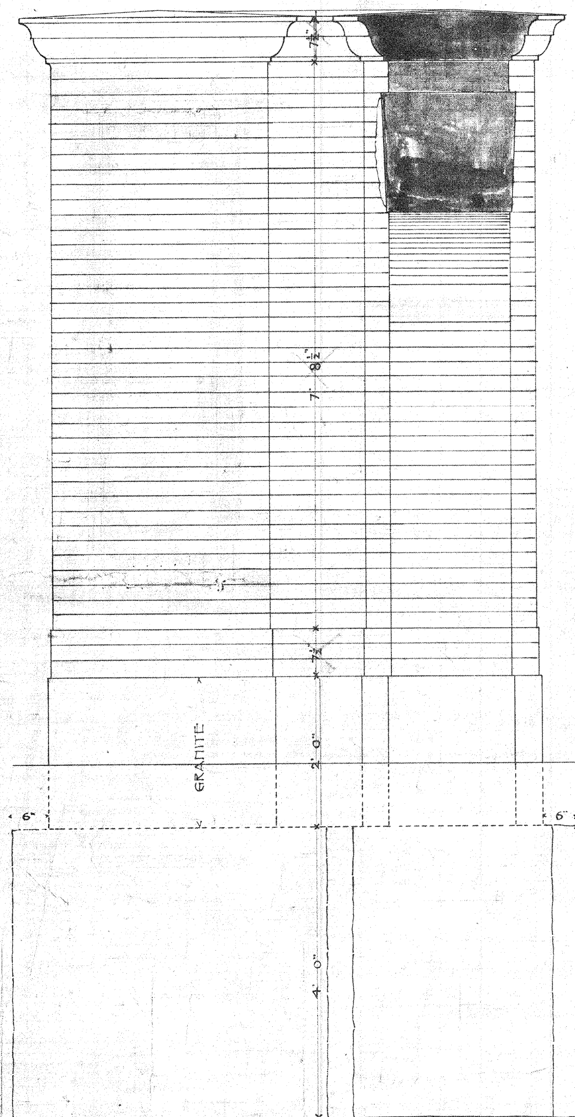
SECTION THROUGH SIDE ENTRANCE LOOKING WEST
