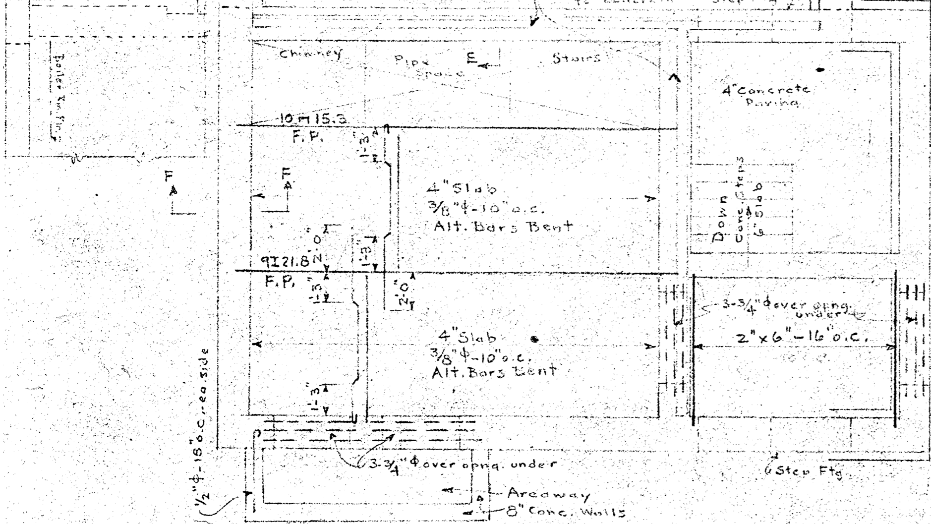
FIRST FLOOR FRAMING Scale: 1/4" = 1'-0"
