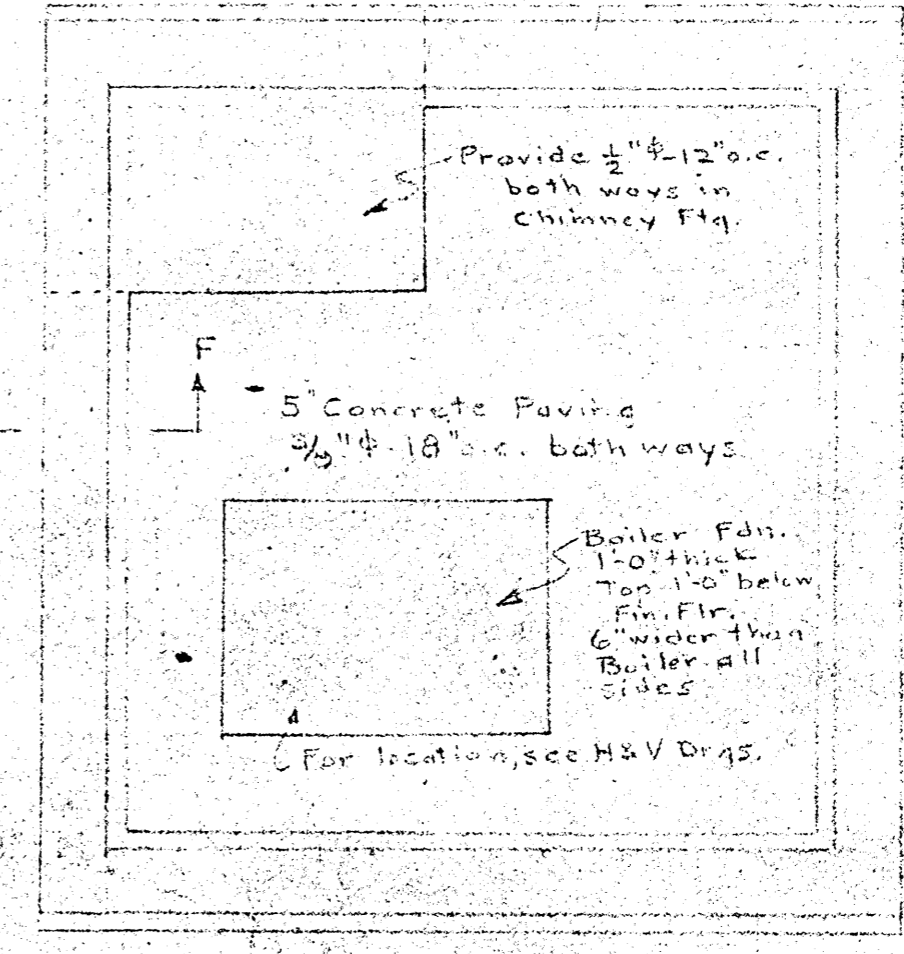
BOILER ROOM FLOOR Scale: 1/4" = 1'-0"
