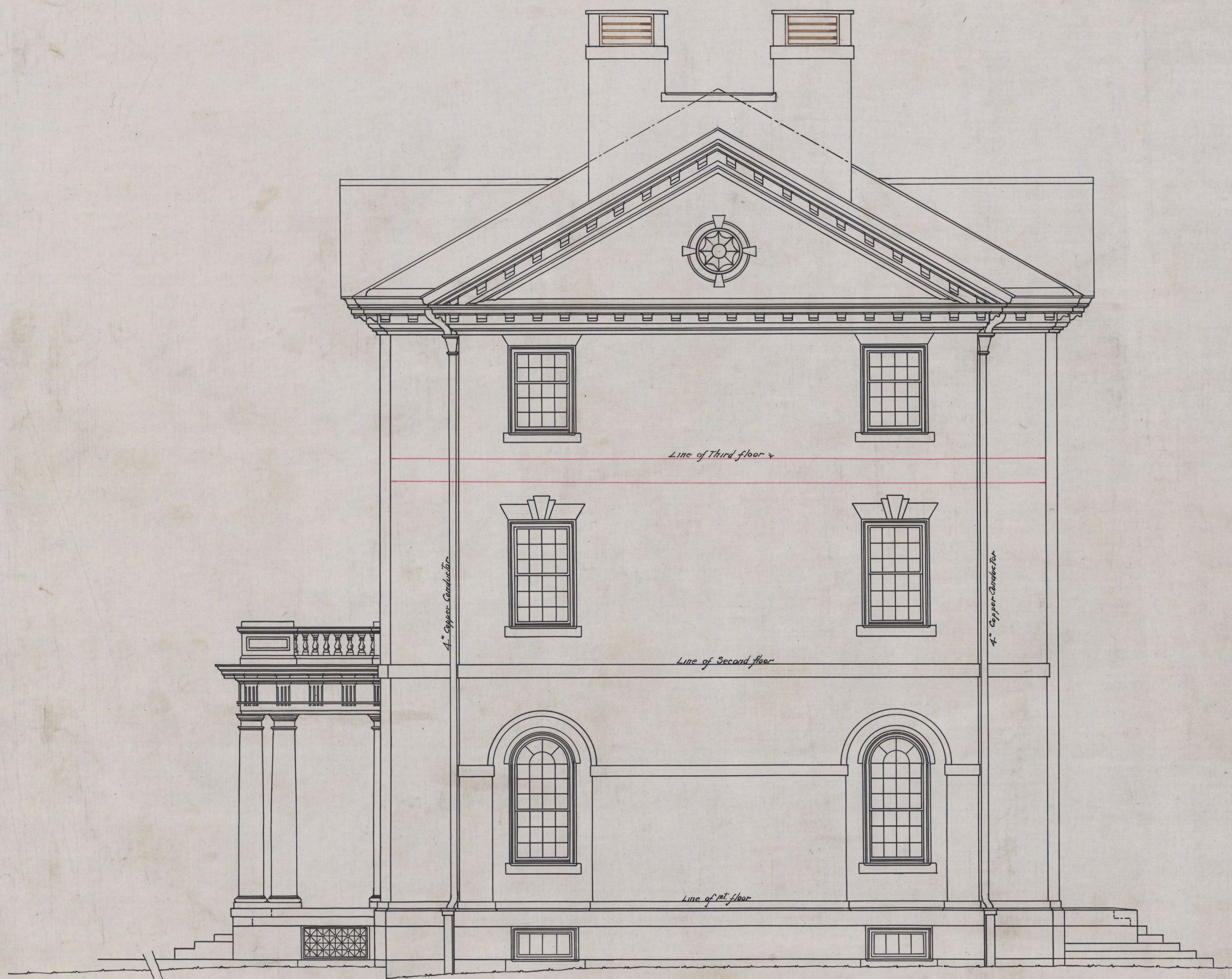
• WEST • ELEVATION •
