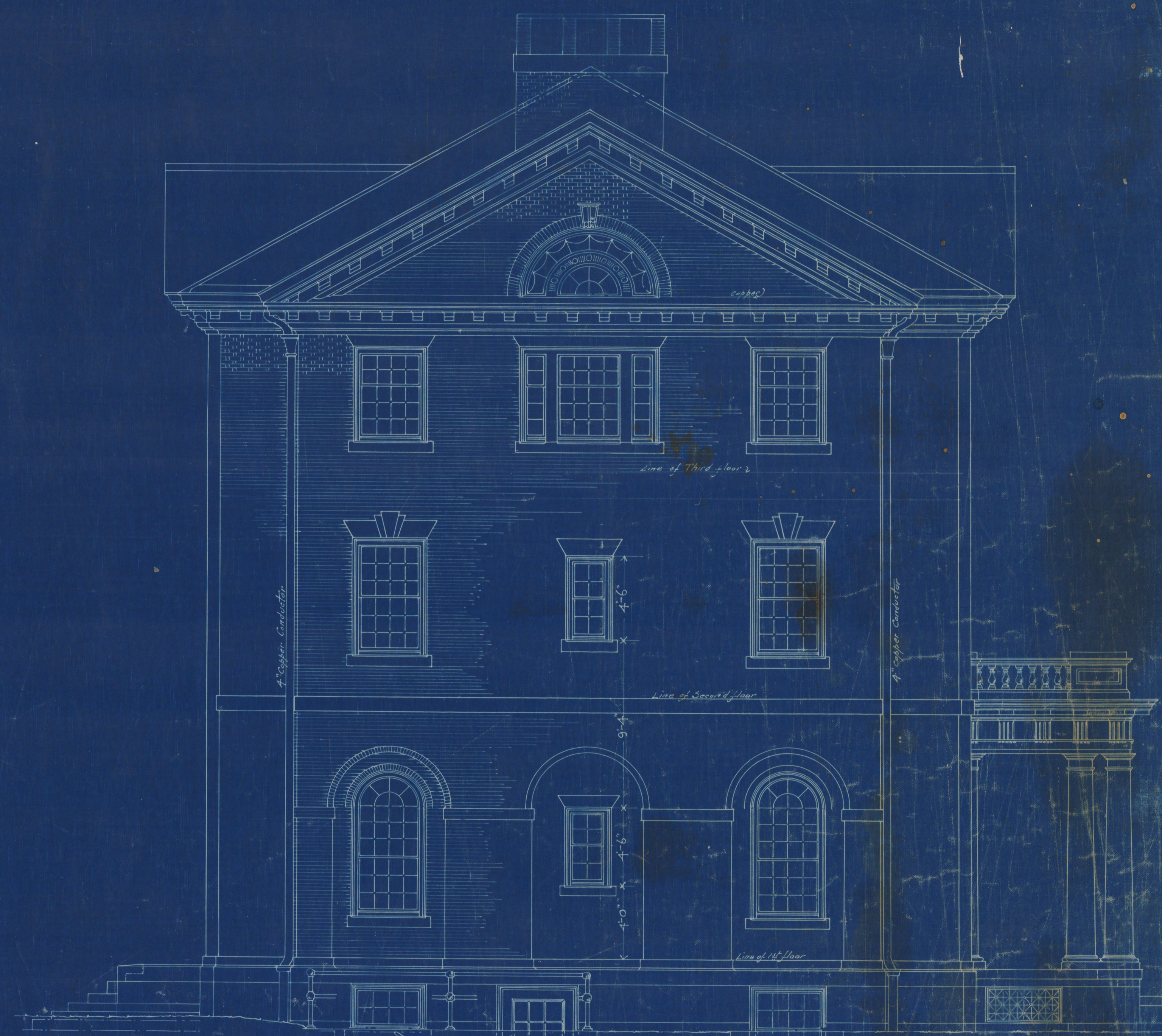
EAST ELEVATION
